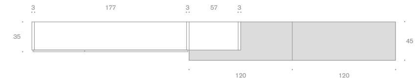
SP025 L/W 423 | H 164 | P/D 35-45
