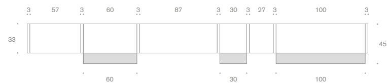
SP027 L/W 382 | H 164 | P/D 33-45
