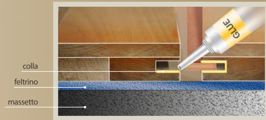
FLOATING INSTALLATION
