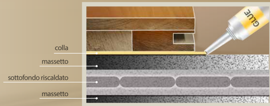
HEATED FLOOR INSTALLATION
