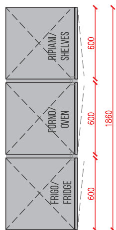
PROFILO AMARI AMARI PROFILE
