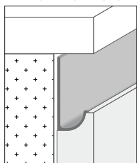
PROFILO JAY SULLE BASI JAY PROFILE FOR BASE UNITS
