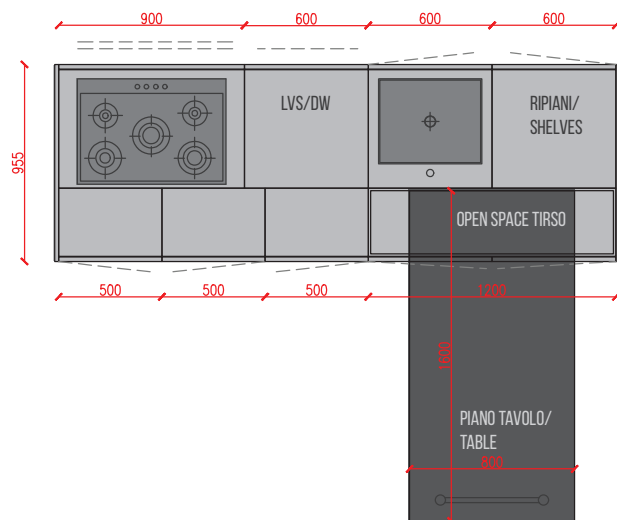
PROFILO SEMPLICE SULLE BASI SIMPLE PROFILE FOR BASE UNITS
